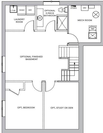
BASEMENT CORNER MODEL • CAMDEN ROW
